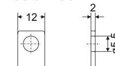
Pole terminals
